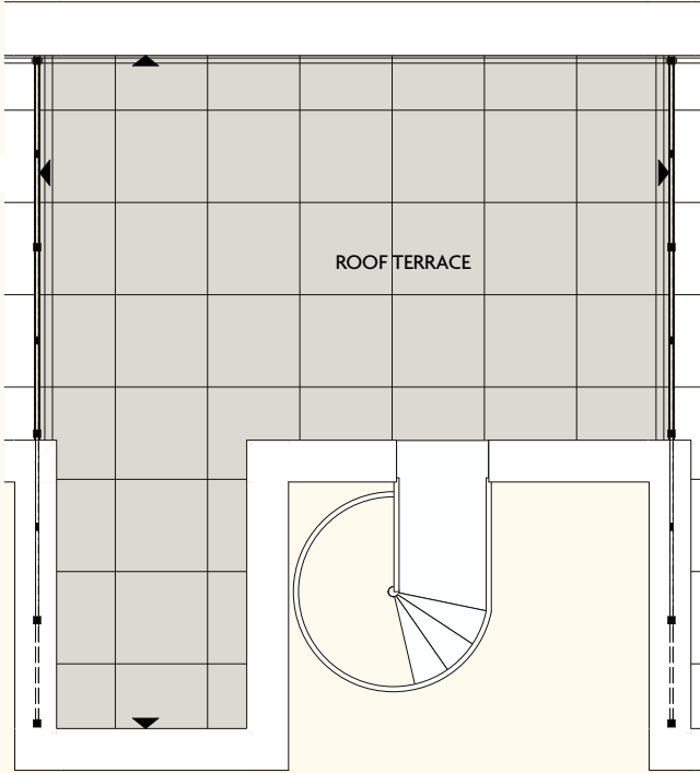
THIRD FLOOR
