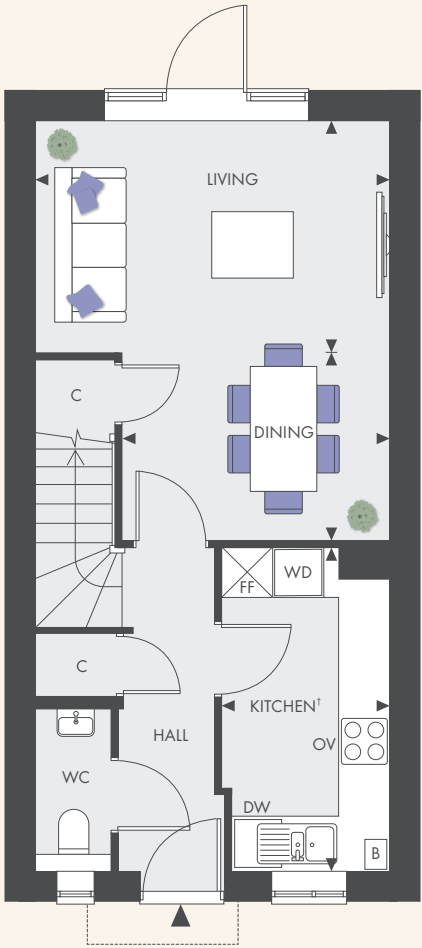
2 BEDROOM MID TERRACE HOUSE Layout applies to plots 300, 305, 308
