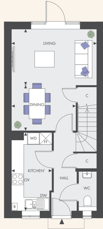
2 BEDROOM END TERRACE HOUSE Layout applies to plots 299, 301*, 304, 306*, 307, 309*
