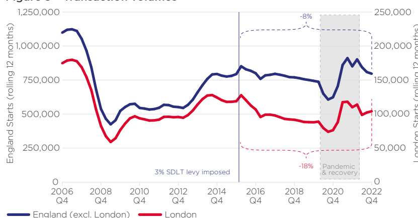
Figure 3 – Transaction volumes
