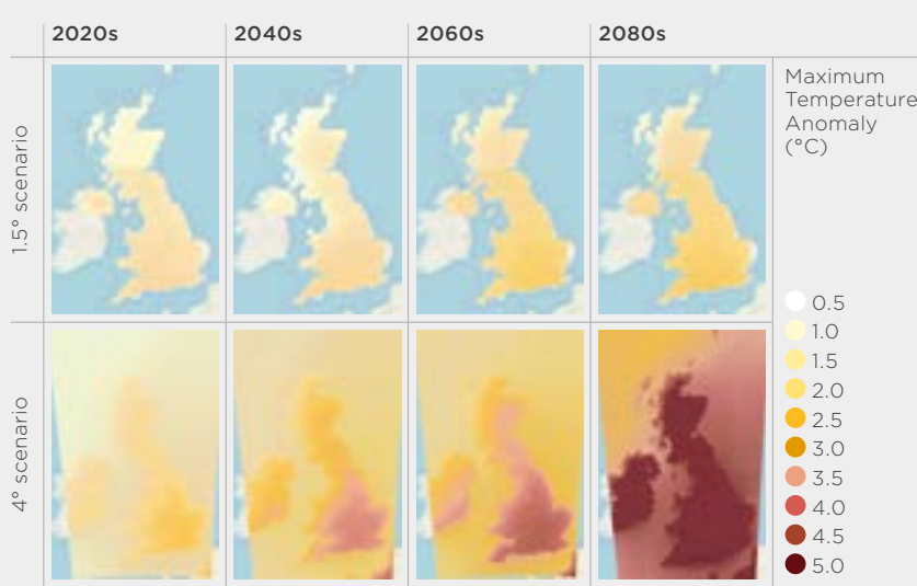
Figure 1: UK maximum temperature anomalies under a 1.5°C and 4°C scenario Temperature variance measured against the 1981 – 2000 baseline, UKCP18 projections (June – August)
